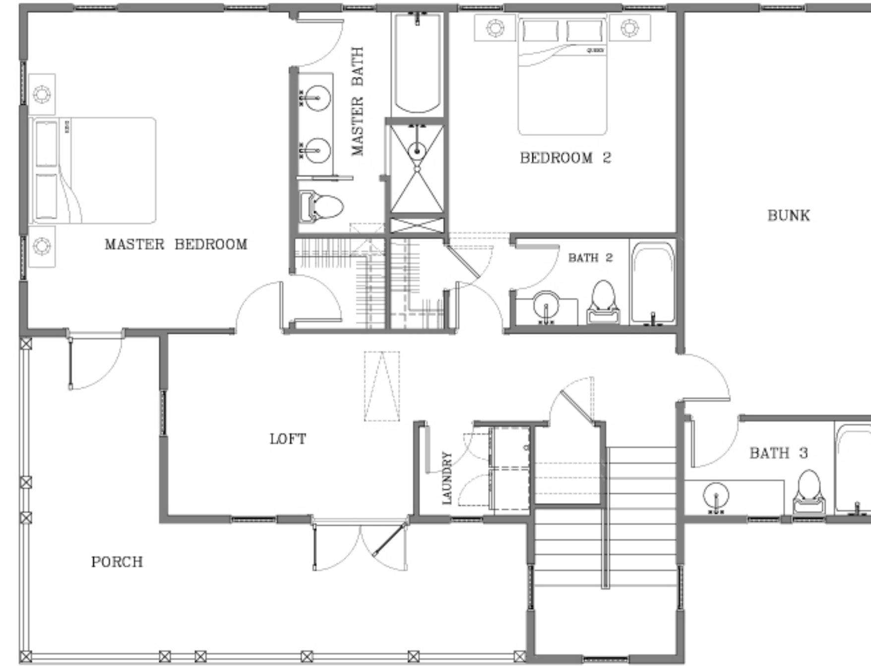
Second Floor
