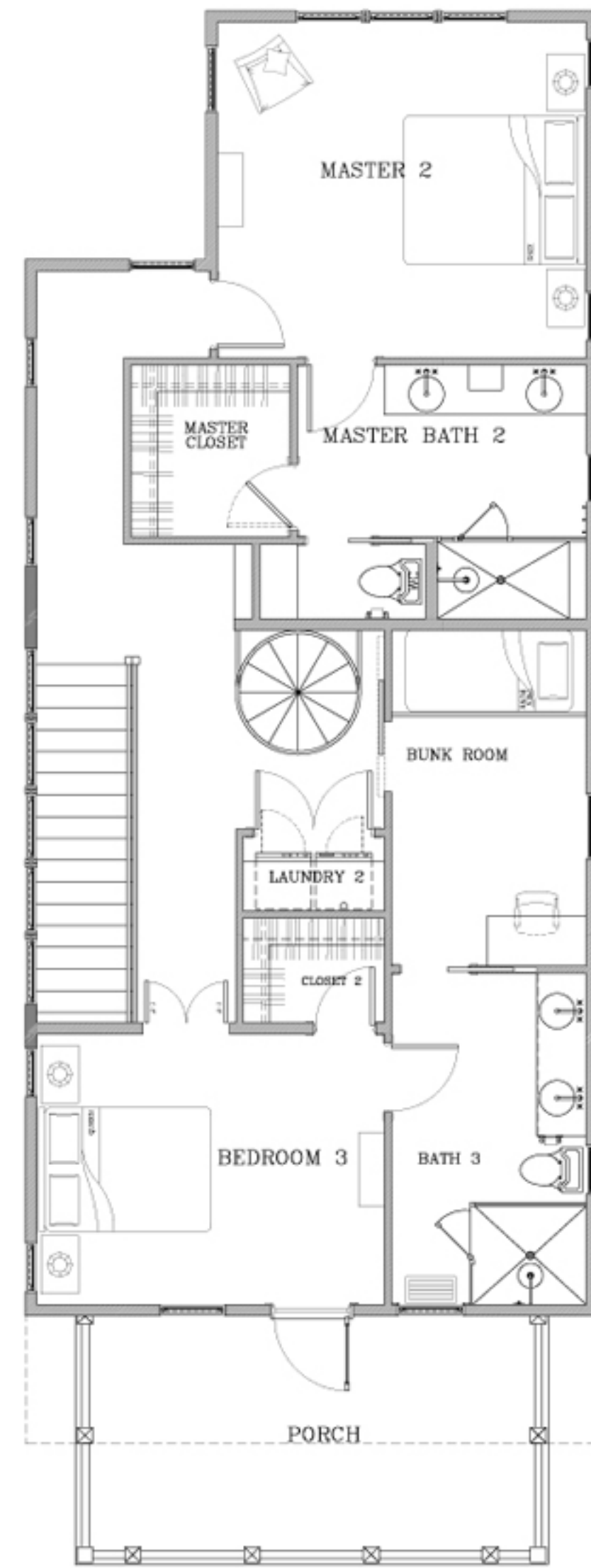
Second Floor
