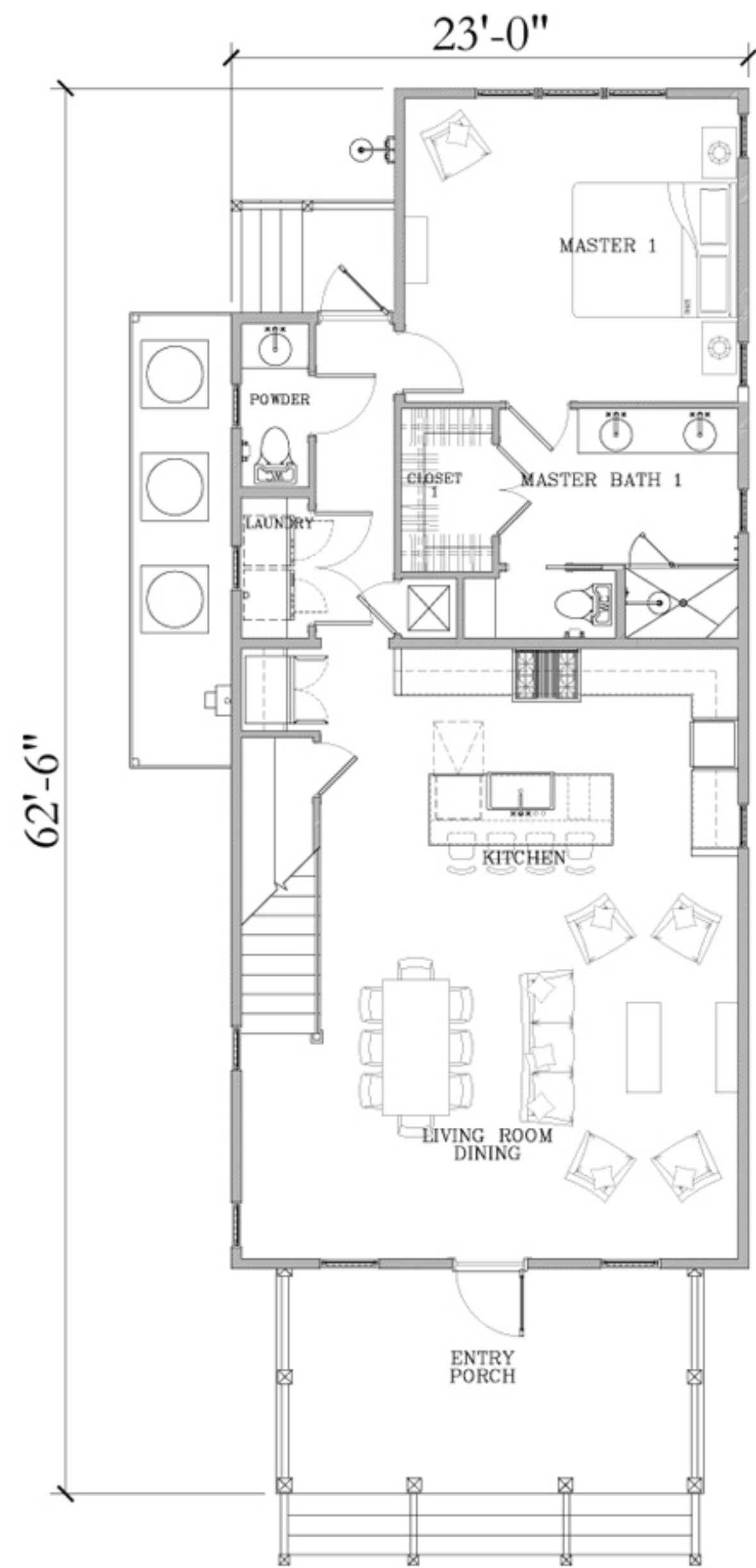
First Floor
